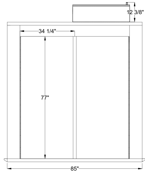
SOIL-SIDE VIEW
