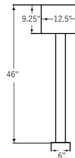
PEDESTAL HMI
